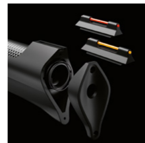
Interchangeable front sight (S3 Suppressor - Sport) with red and orange fiber optic
